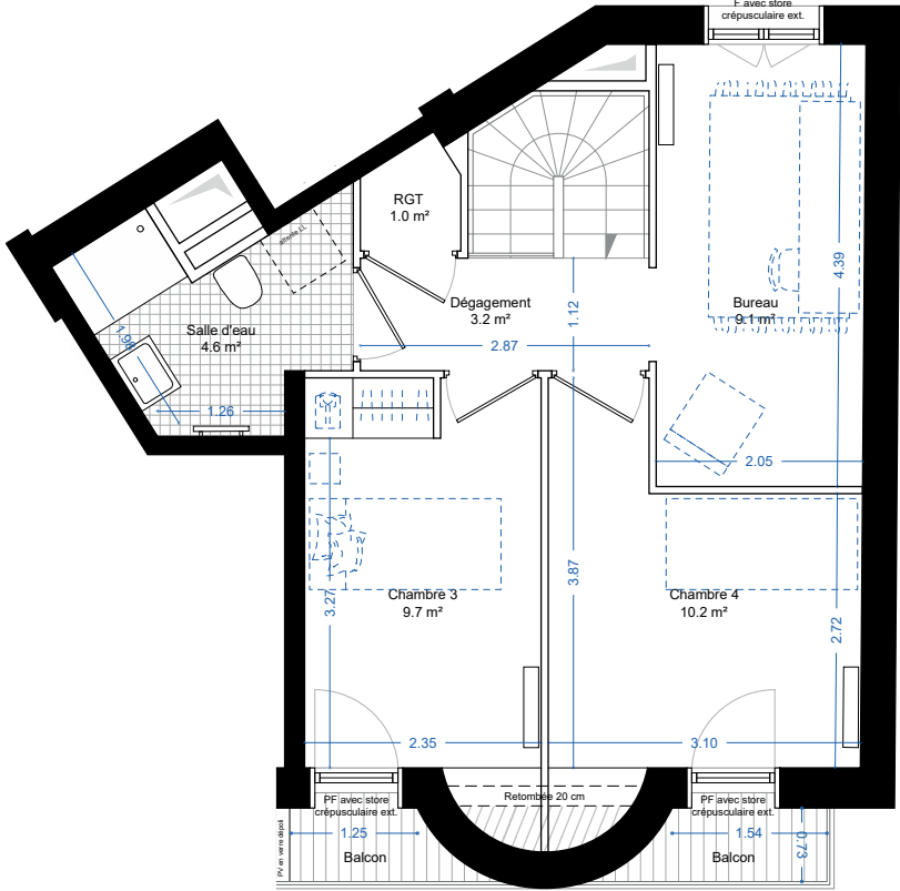
R+5
